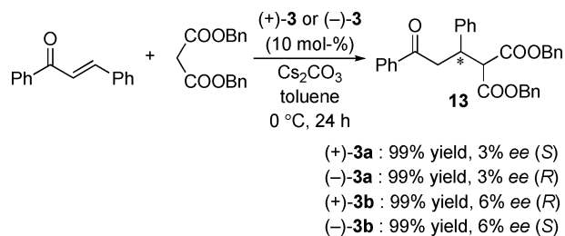
Scheme 6. Asymmetric Michael addition reaction of malonate catalysed by 3 under phase-transfer conditions.
