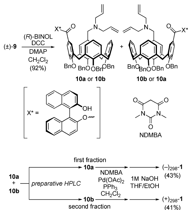
Scheme 2. Resolution of an inherently chiral calix[4]arene amino acid.
