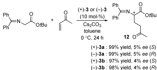
Scheme 5. Asymmetric Michael addition reaction of a glycine derivative catalysed by 3 under phase-transfer conditions.
