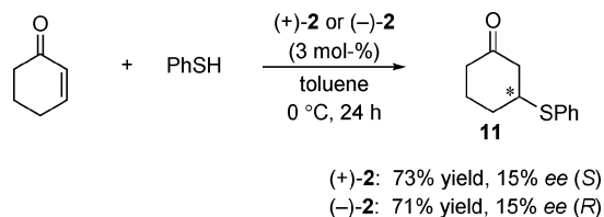
Scheme 4. Asymmetric Michael addition reaction of thiophenol catalysed by 2 .
