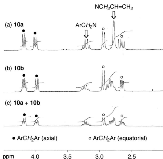
Figure 2. A section of the ^1\text{H} NMR spectra of calix[4]arenes 10a (a) and 10b (b), and mixture of 10a and 10b (c) in \text{CDCl}_3 at 27^\circ\text{C} .
