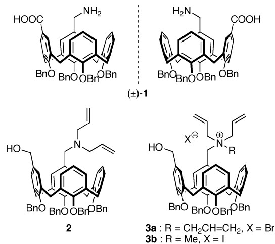
Figure 1. Inherently chiral calix[4]arene amino acid and its derivatives.
