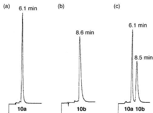
Figure 3. HPLC chromatographs of 10a (a) and 10b (b), and a mixture of 10a and 10b (c) [column: SUMICHIRAL OA-4800 ( 0.46 \times 25 cm), eluent: \text{CHCl}_3 /hexane (80:20), flow rate: 1.0 \text{ mL min}^{-1} ].
