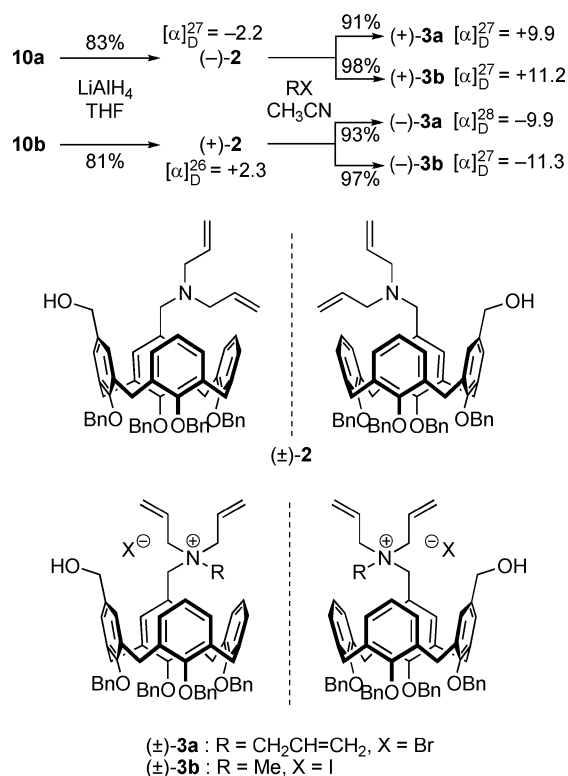
Scheme 3. Synthesis of inherently chiral calix[4]arenes 2 and 3 .
