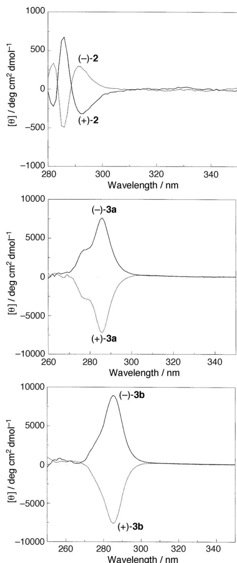
Figure 5. CD spectra of enantiomers of calix[4]arenes 2 , 3a and 3b in \text{CHCl}_3 .
