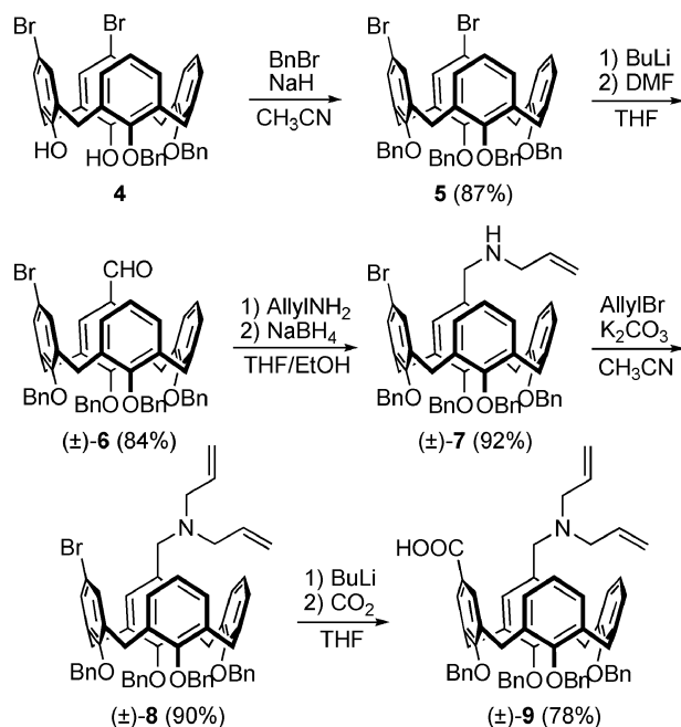
Scheme 1. Synthesis of N -protected calix[4]arene amino acid 9 .
