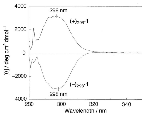
Figure 4. CD spectra of the enantiomers of calix[4]arene amino acid 1 in \text{CHCl}_3 .
